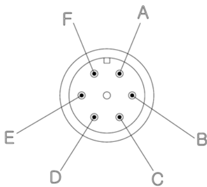
Electrical Connection
